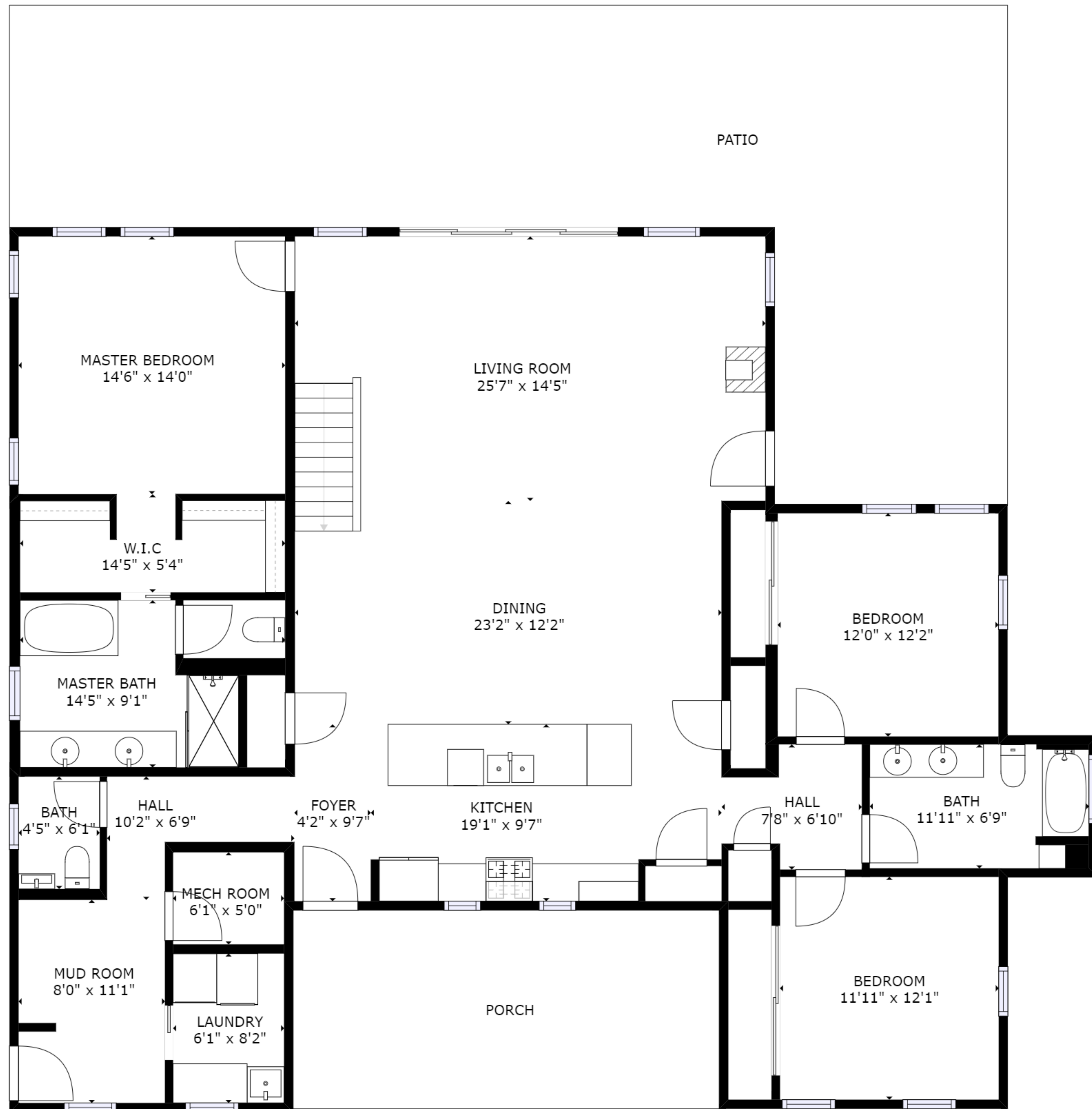
FLOOR 1
